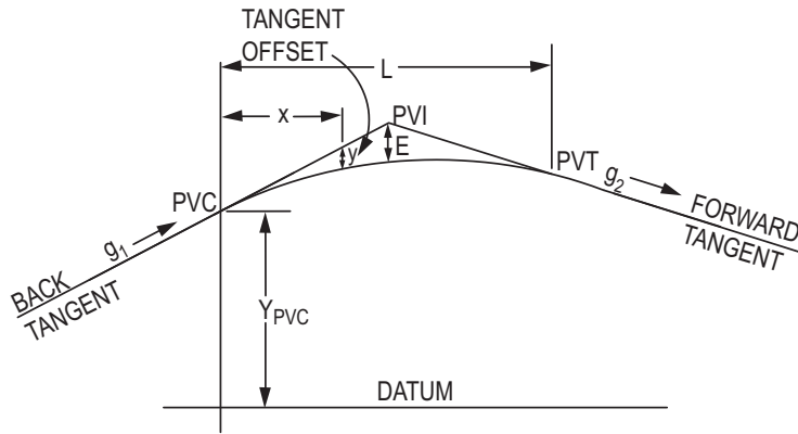
VERTICAL CURVE FORMULAS NOT TO SCALE
