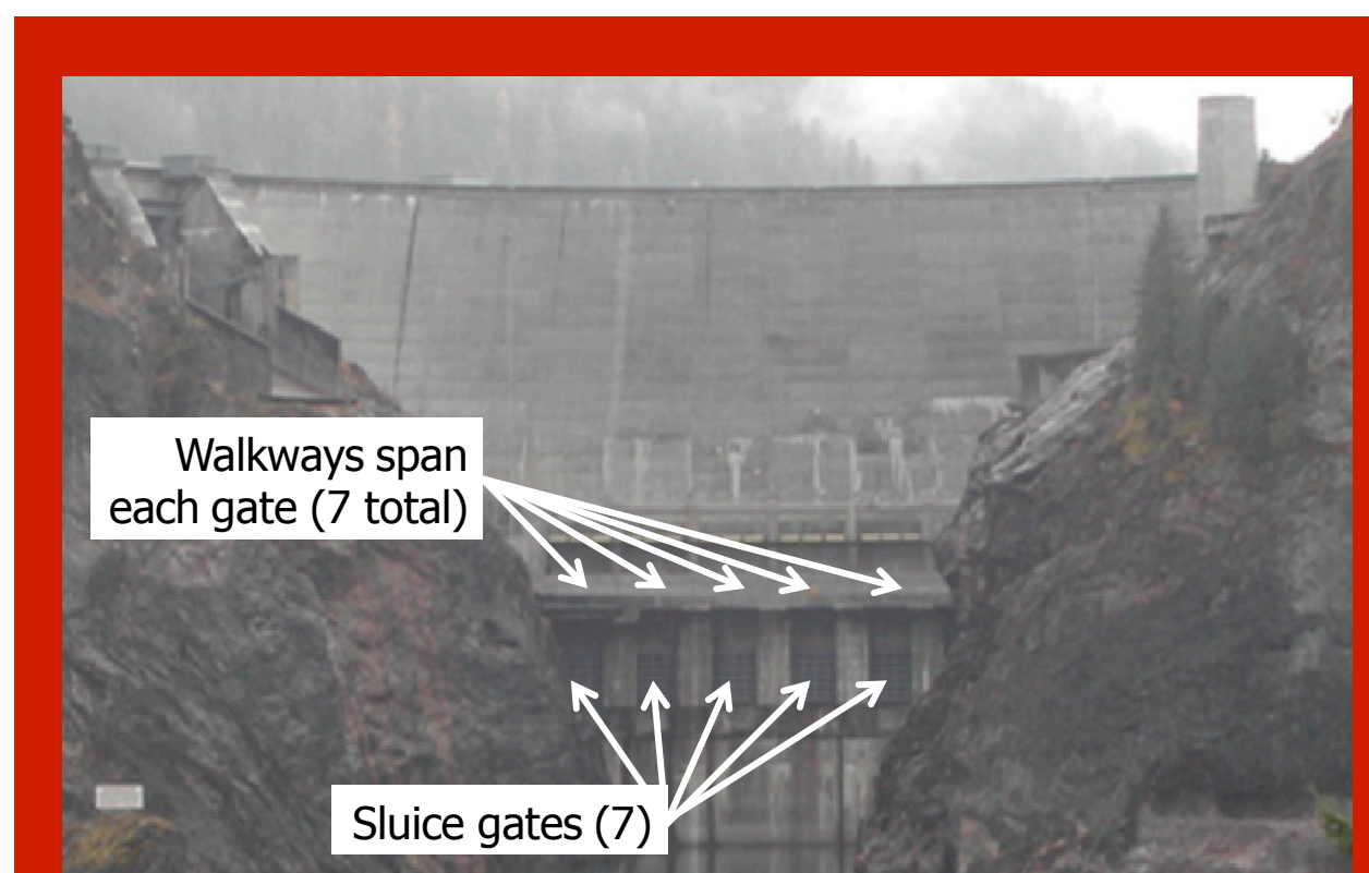
Dam with seven walkways
